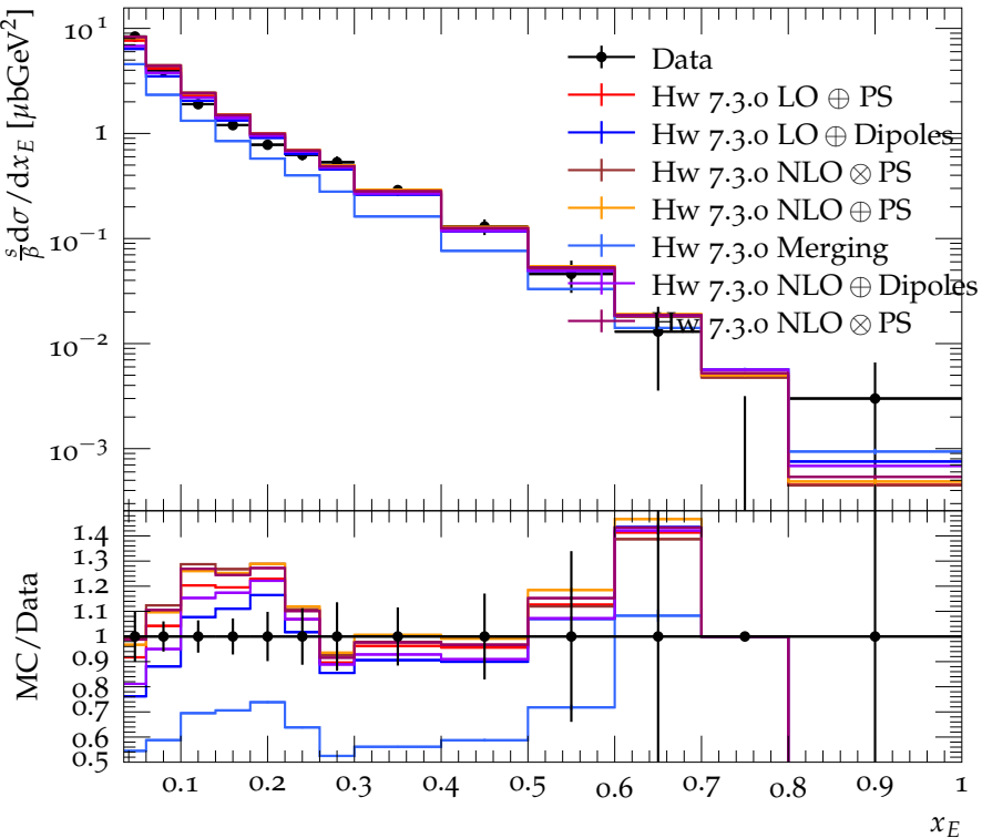
K^0 spectrum at 29 GeV
