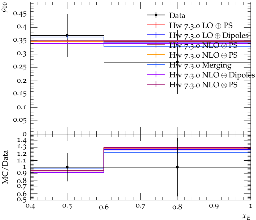
\rho_{00} for D^* production, helicity-beam frame
