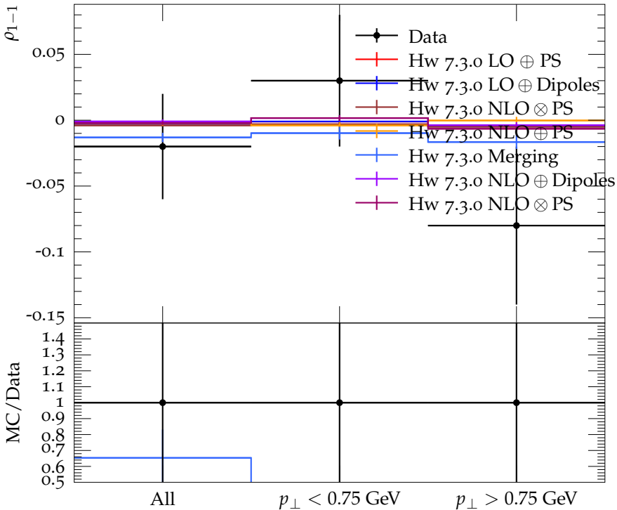
\rho_{1-1} for D^* production, helicity-quark frame, ( x_E > 0.4 )
