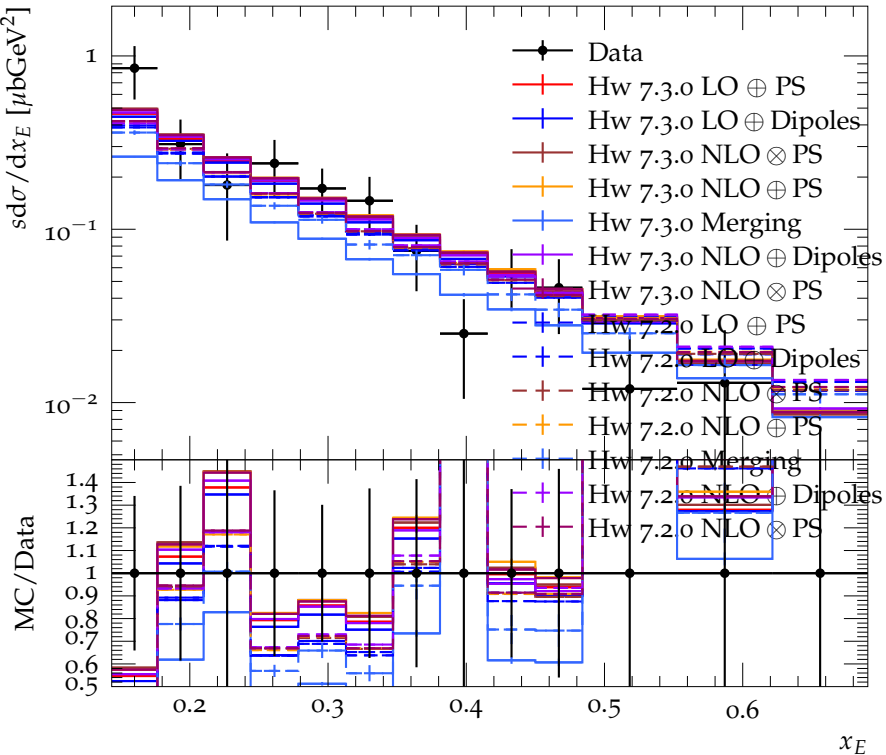
\eta spectrum at E_{\text{CMS}} = 29 GeV
