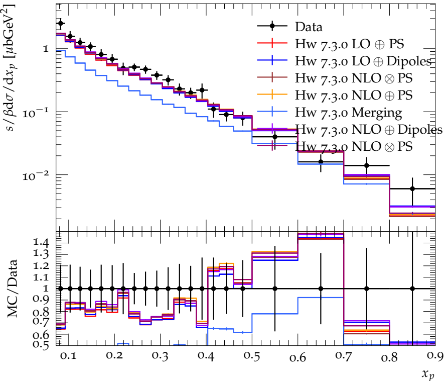
Scaled momentum for \rho^0 at 29 GeV
