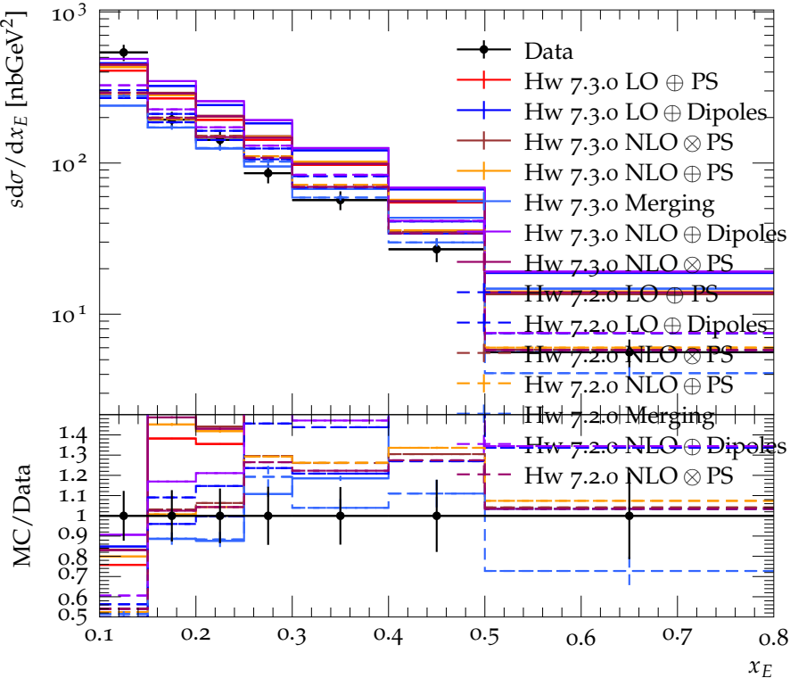
\Lambda spectrum at E_{\text{CMS}} = 29 \text{ GeV}
