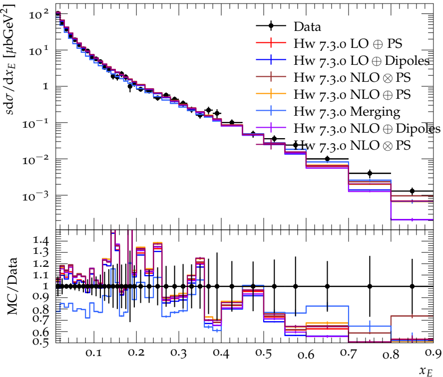
\gamma scaled energy spectrum at 34.4 GeV
