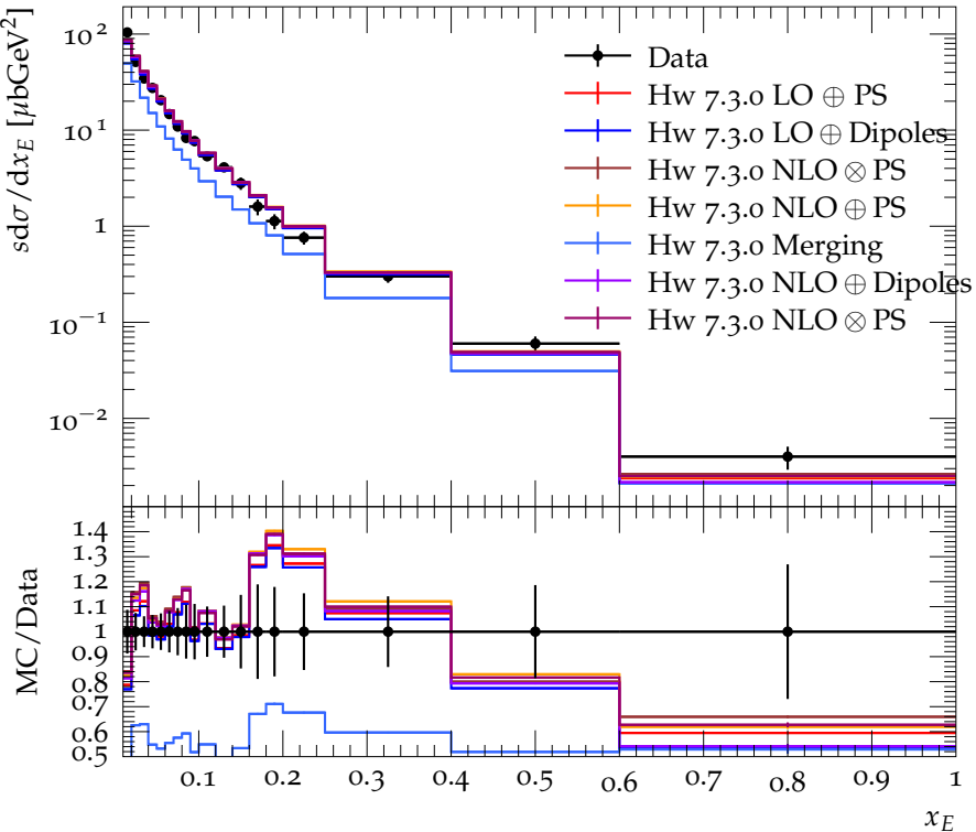
\gamma scaled energy spectrum at 22.5 GeV
