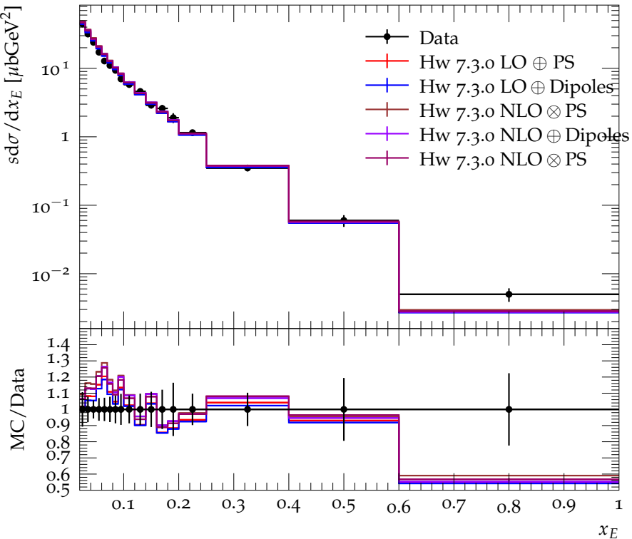
\gamma scaled energy spectrum at 14 GeV
