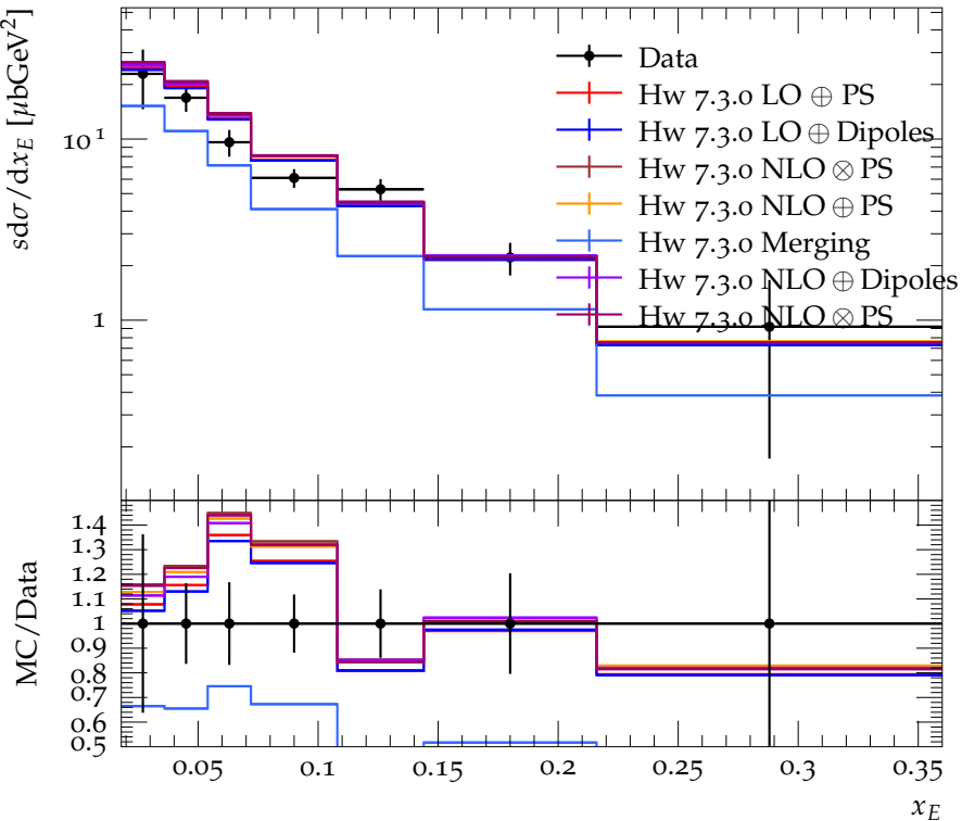
\pi^0 scaled energy spectrum at 22.5 GeV
