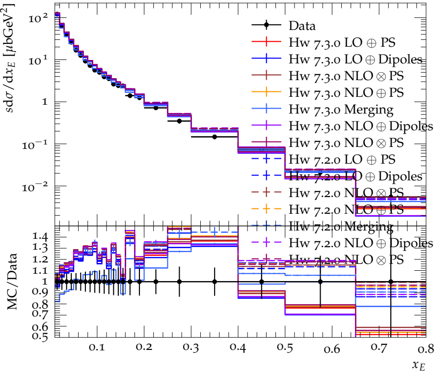
\gamma scaled energy spectrum at 44 GeV
