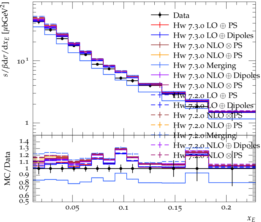
\pi^0 scaled energy spectrum at 35 GeV
