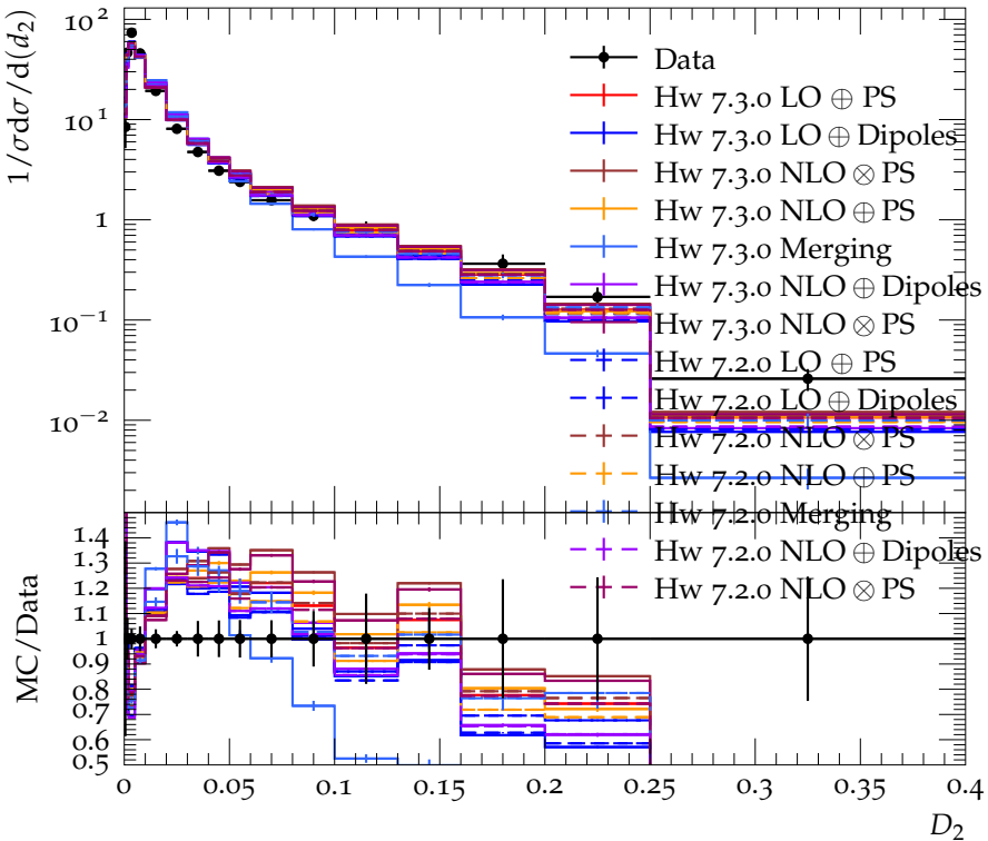
Differential 2-Jet rate (Durham), \sqrt{s} = 35 GeV
