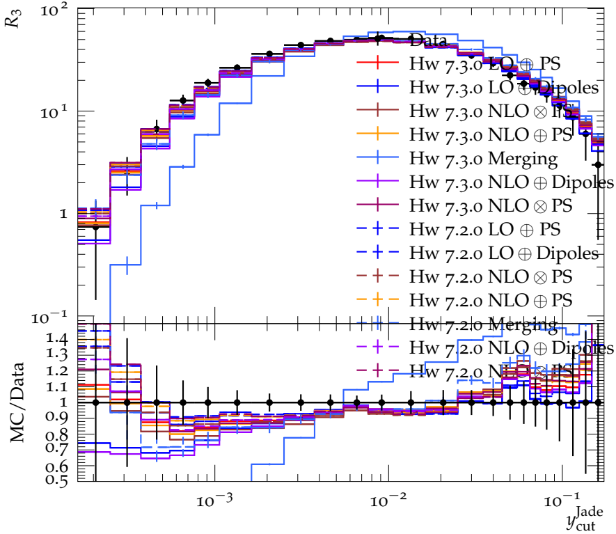
Integrated 3-jet rate with Jade algorithm (183 GeV)
