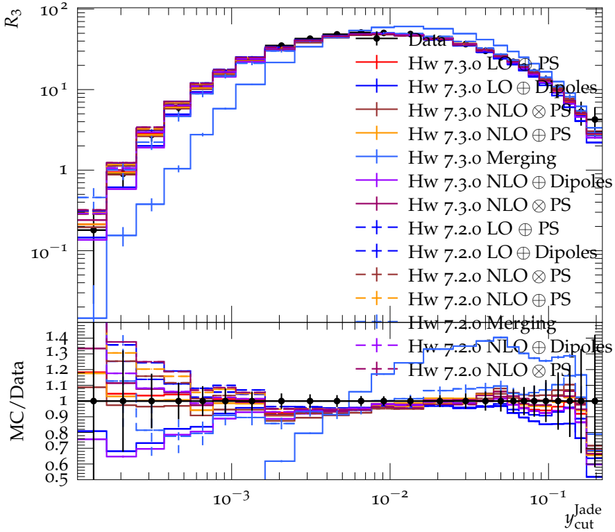
Integrated 3-jet rate with Jade algorithm (189 GeV)
