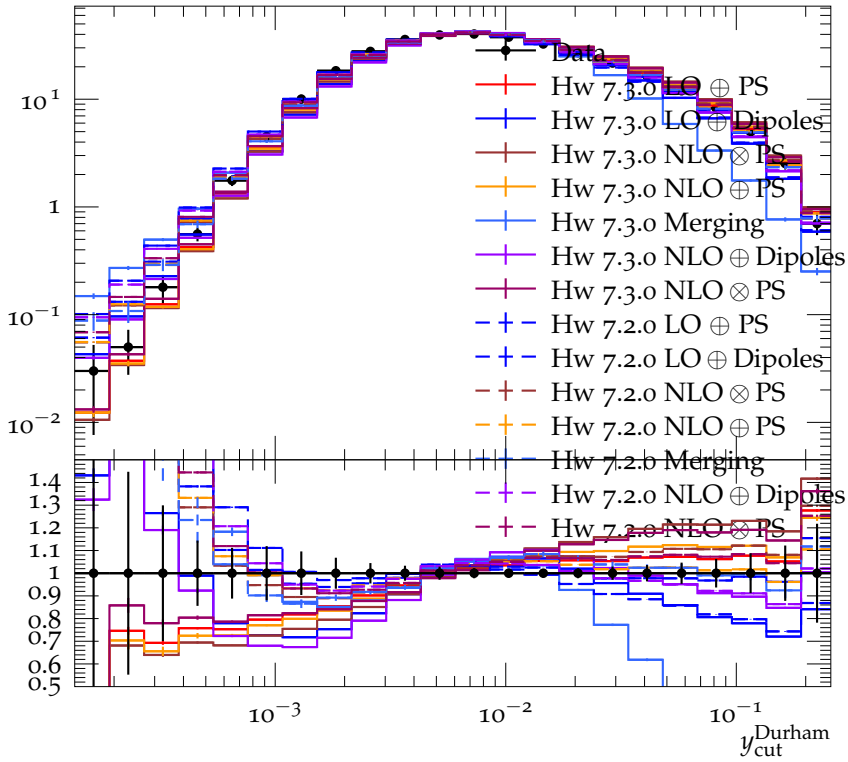
Integrated 3-jet rate with Durham algorithm (35 GeV)
