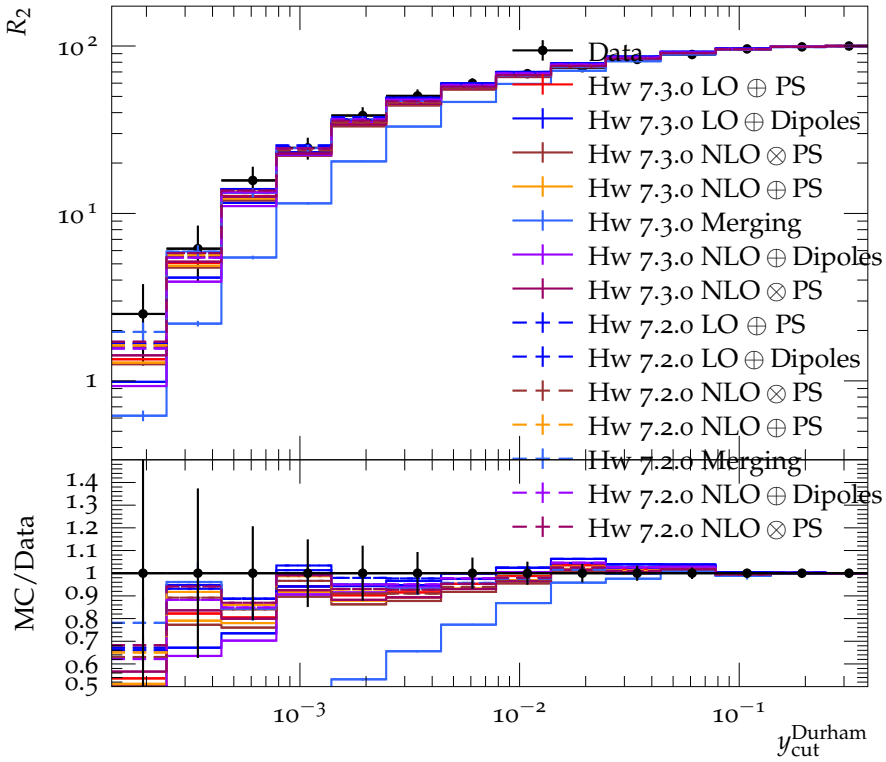
Integrated 2-jet rate with Durham algorithm (161 GeV)
