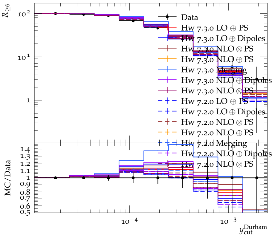
Integrated \geq 6 -jet rate with Durham algorithm (161 GeV)
