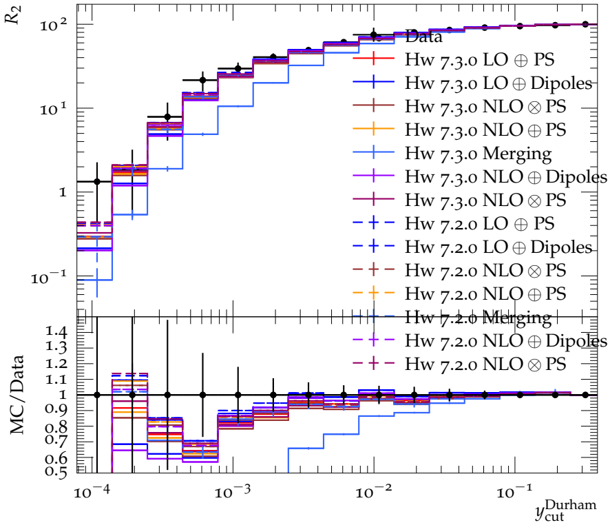
Integrated 2-jet rate with Durham algorithm (172 GeV)
