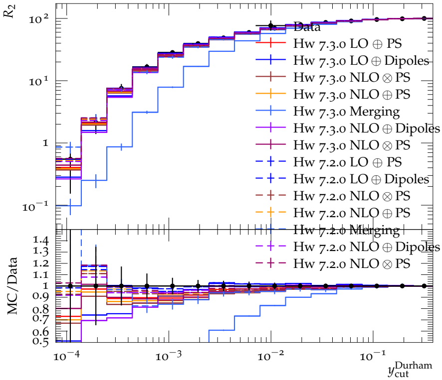
Integrated 2-jet rate with Durham algorithm (183 GeV)
