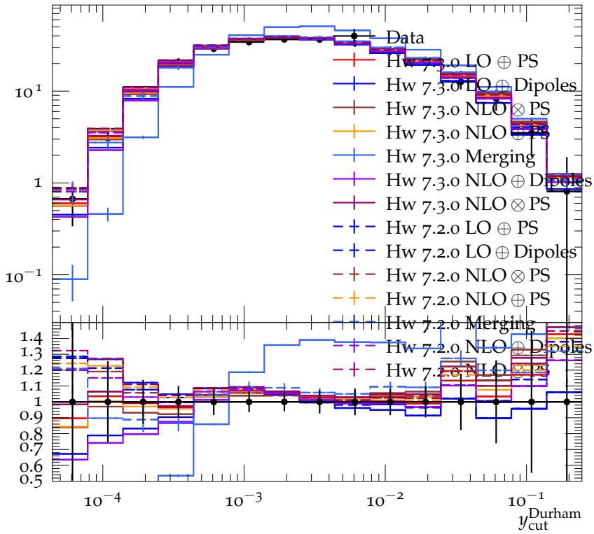
Integrated 3-jet rate with Durham algorithm (183 GeV)
