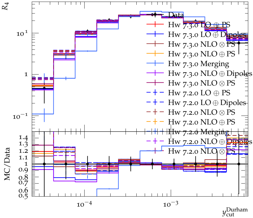
Integrated 4-jet rate with Durham algorithm (183 GeV)
