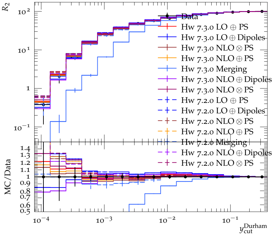
Integrated 2-jet rate with Durham algorithm (189 GeV)
