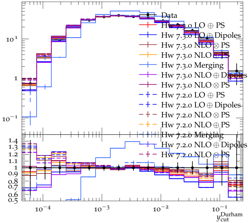
Integrated 3-jet rate with Durham algorithm (189 GeV)
