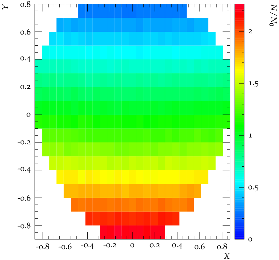
Dalitz plot for \eta \rightarrow \pi^+ \pi^- \pi^0
