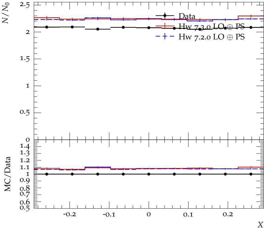
Dalitz plot slice for -0.9 < Y < -0.8
