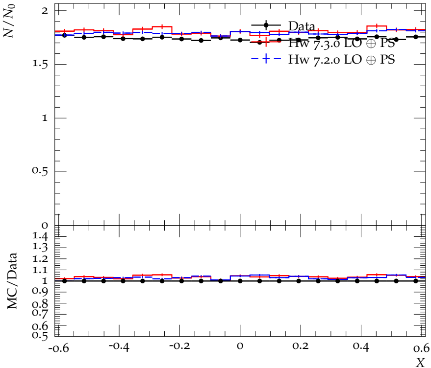
Dalitz plot slice for -0.6 < Y < -0.5
