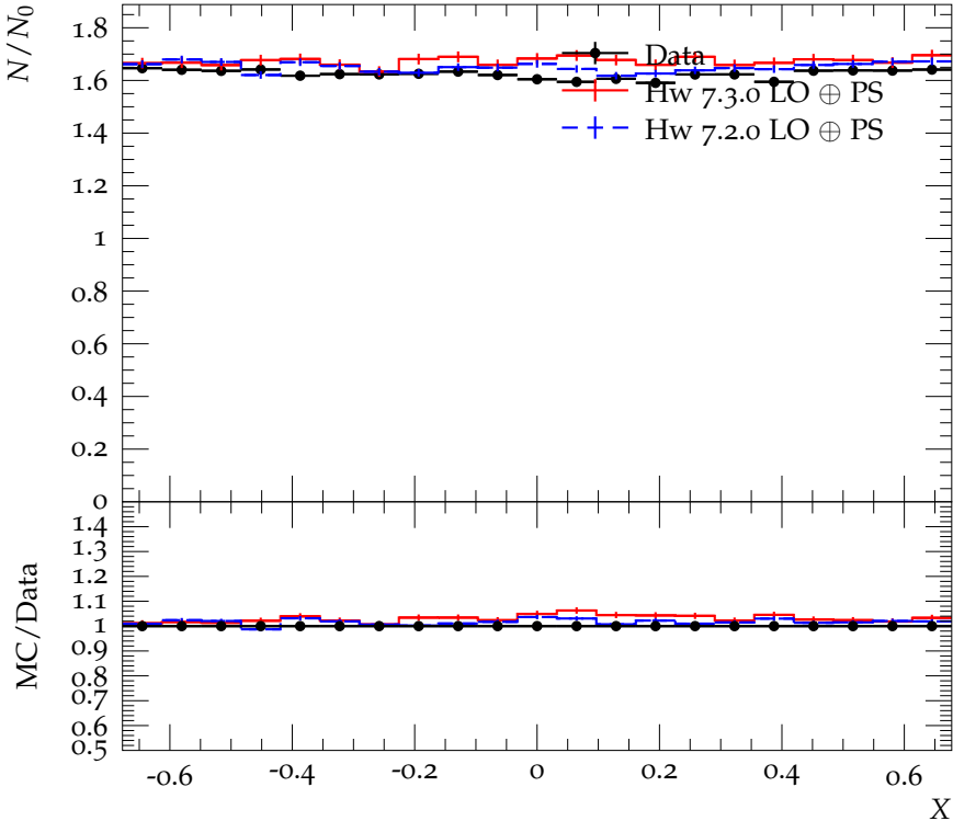
Dalitz plot slice for -0.5 < Y < -0.4
