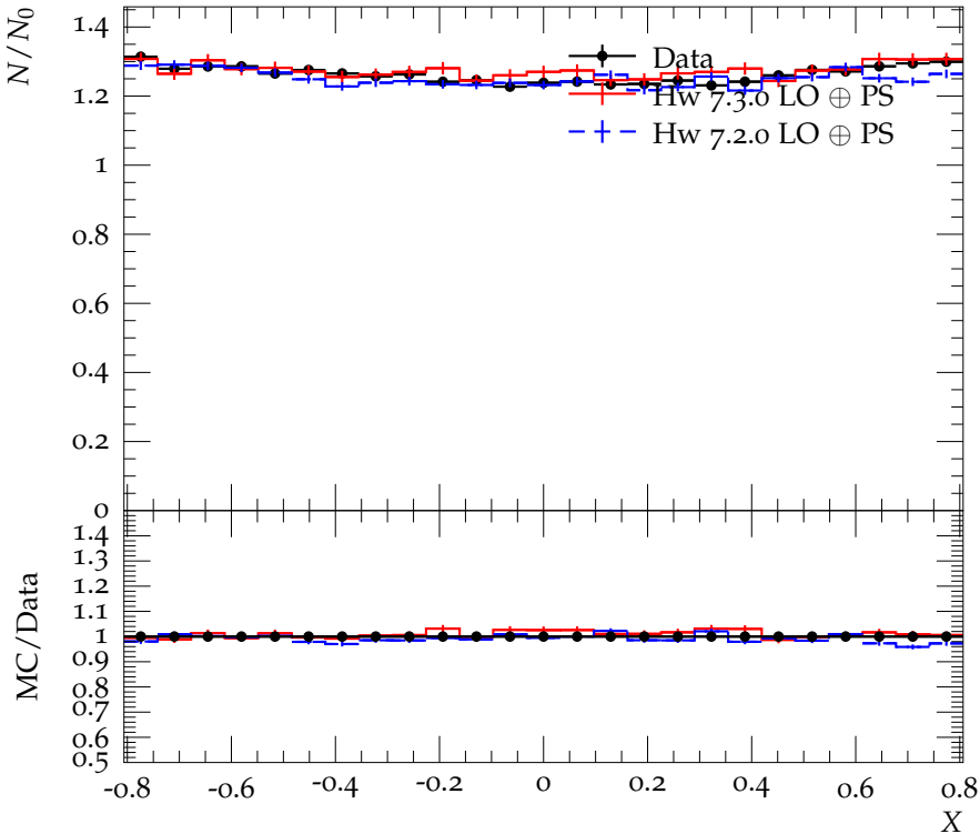
Dalitz plot slice for -0.2 < Y < -0.1
