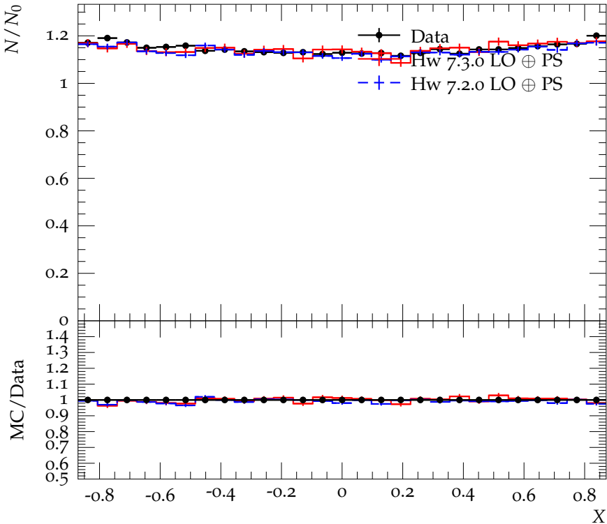
Dalitz plot slice for -0.1 < Y < 0.0
