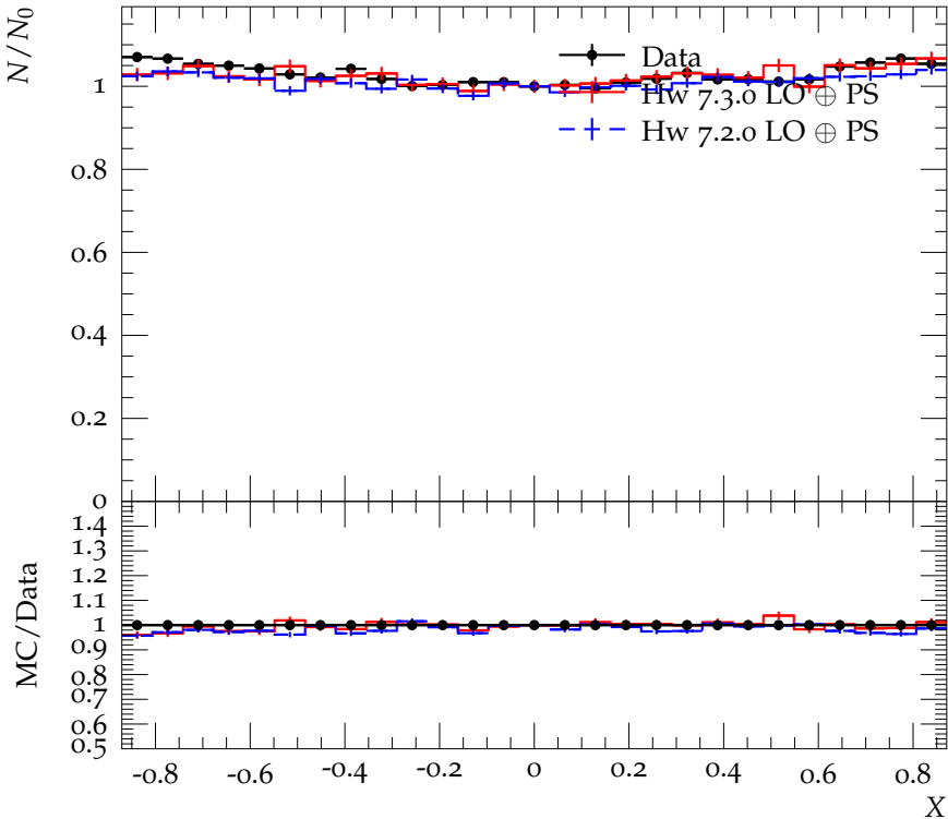
Dalitz plot slice for 0.0 < Y < 0.1
