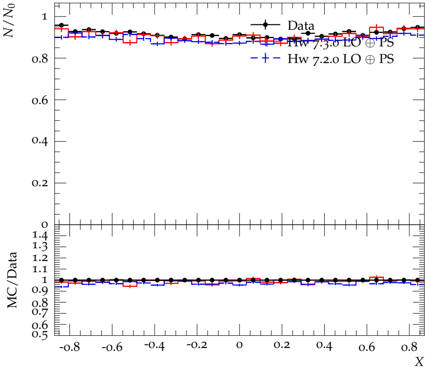
Dalitz plot slice for 0.1 < Y < 0.2
