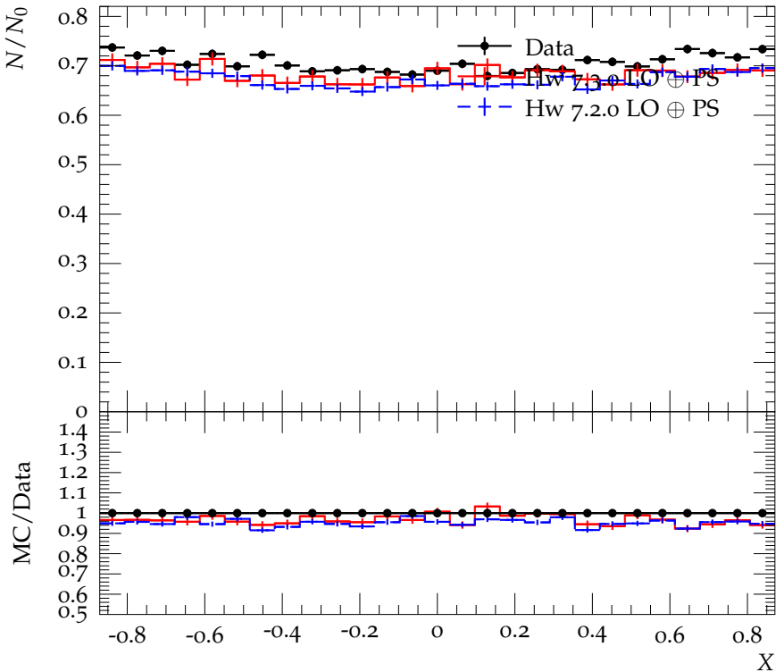
Dalitz plot slice for 0.3 < Y < 0.4
