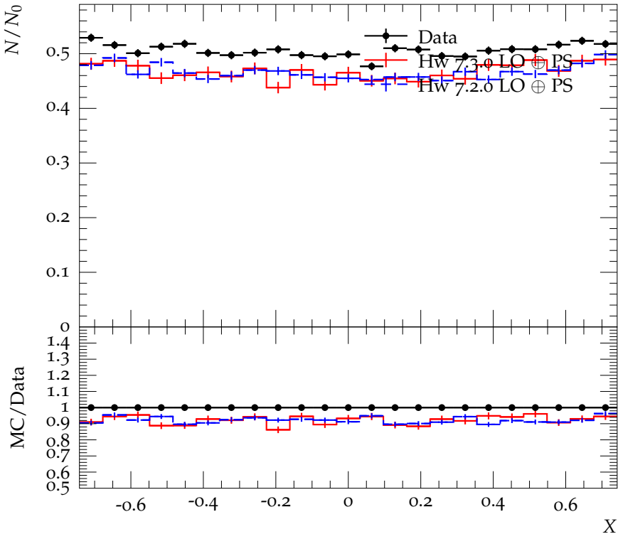
Dalitz plot slice for 0.5 < Y < 0.6
