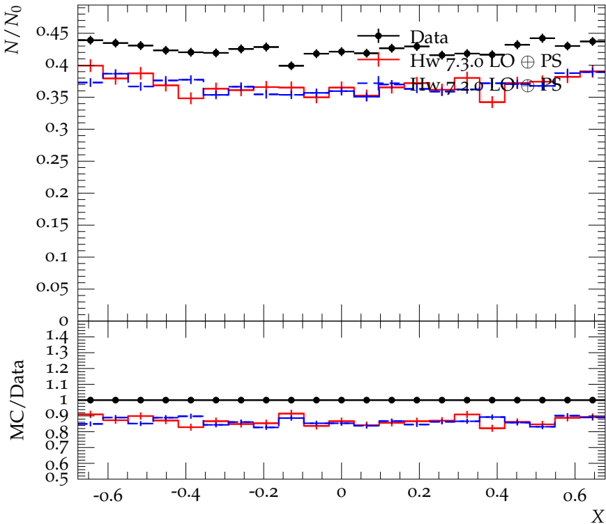
Dalitz plot slice for 0.6 < Y < 0.7
