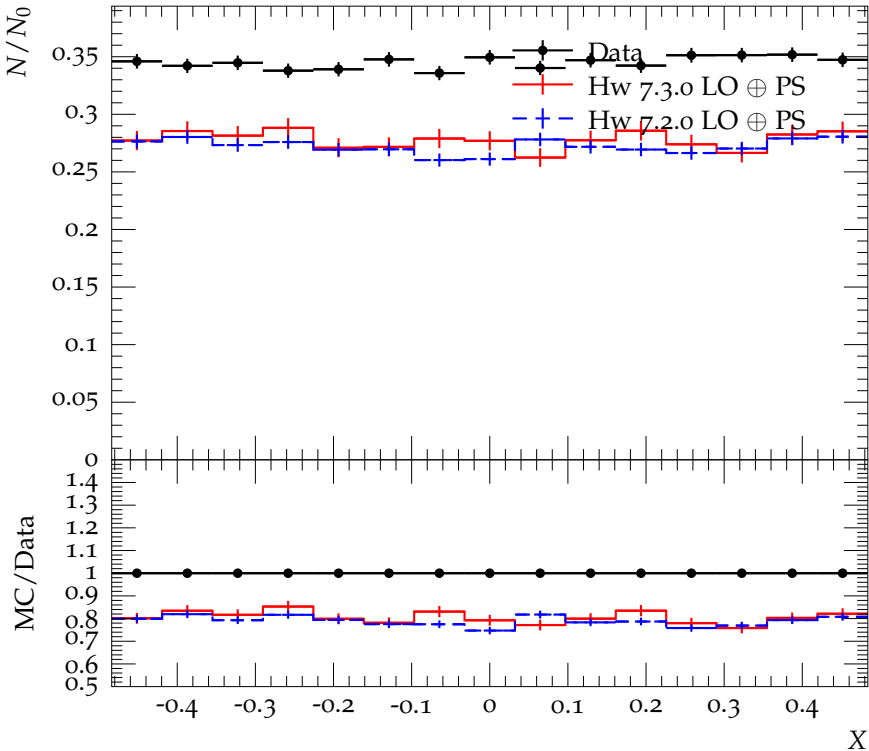
Dalitz plot slice for 0.7 < Y < 0.8
