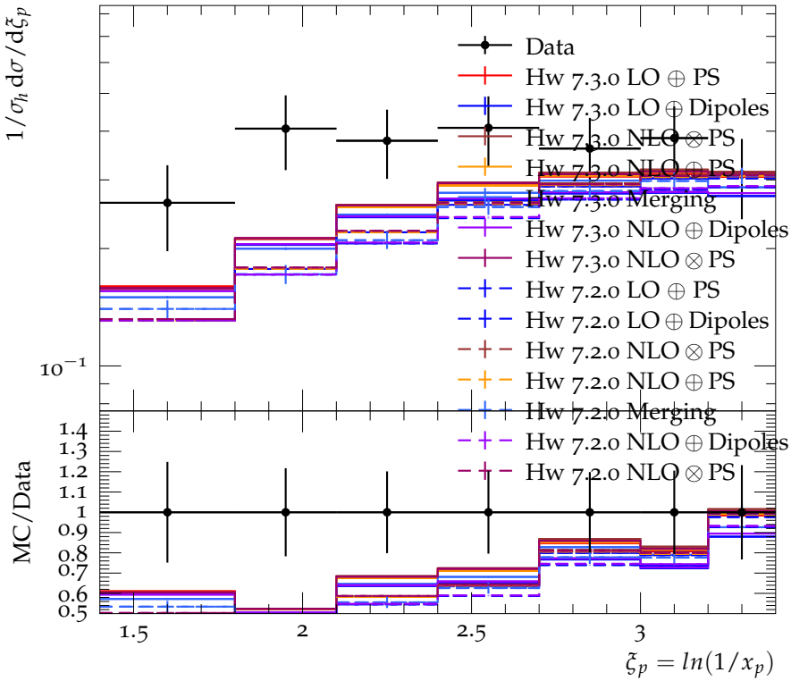
The \xi_p spectrum for inclusive \eta production at the Z^0 resonance
