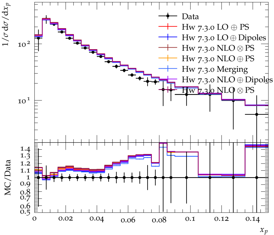
\pi^0 scaled spectrum using HERWIG for corrections
