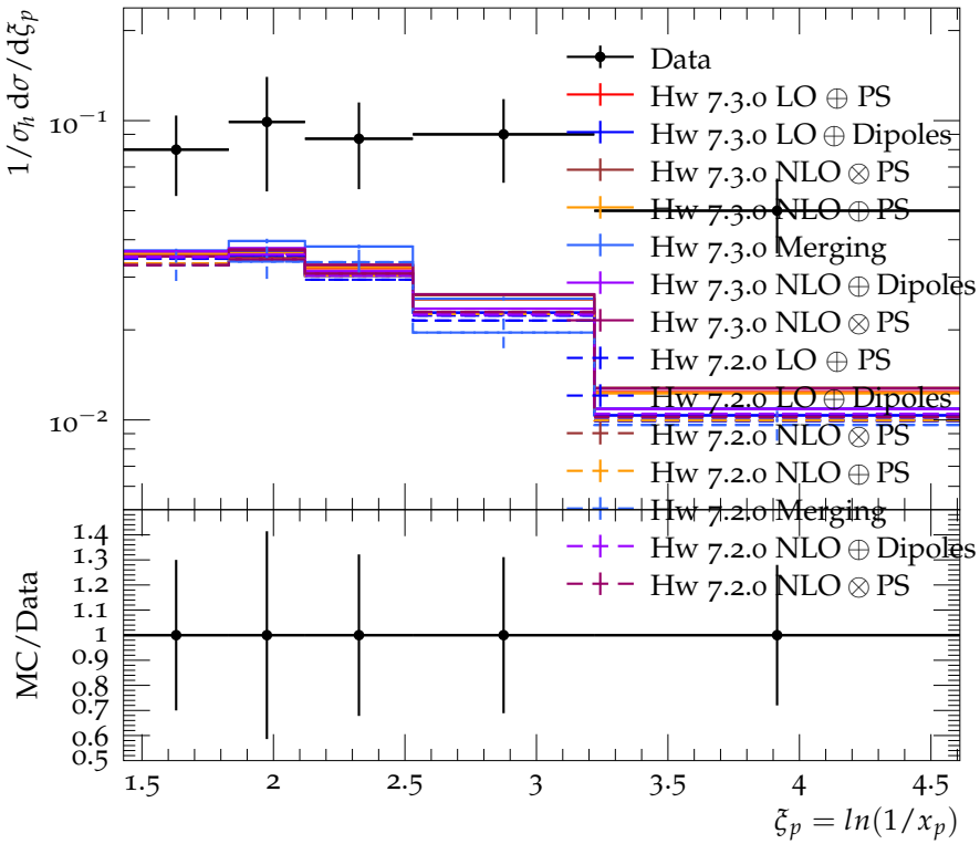
The \xi_p spectrum for \eta' (using \eta' \rightarrow \rho^0 \gamma ) at the Z^0 resonance
