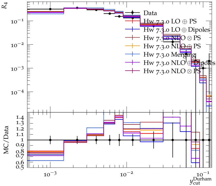
Integrated 4-jet rate with Jade algorithm (130.1 GeV)
