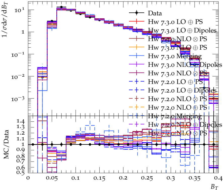
Total jet broadening, b events, at E_{\text{CMS}} = 91.2 GeV
