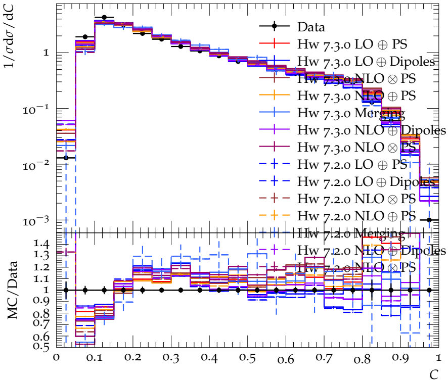
C-parameter, b events, at E_{\text{CMS}} = 91.2 GeV
