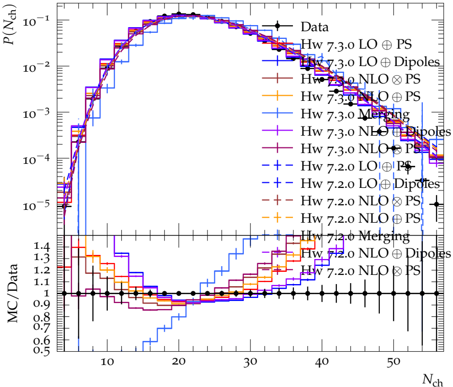
Charged multiplicity, b events, at E_{\text{CMS}} = 91.2 GeV
