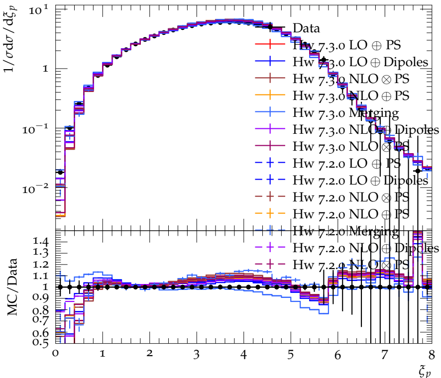
Log of scaled momentum distribution, udsc events, at E_{\text{CMS}} = 91.2
