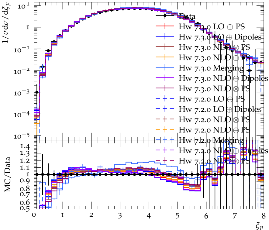
Log of scaled momentum distribution, b events, at E_{\text{CMS}} = 91.2 Ge
