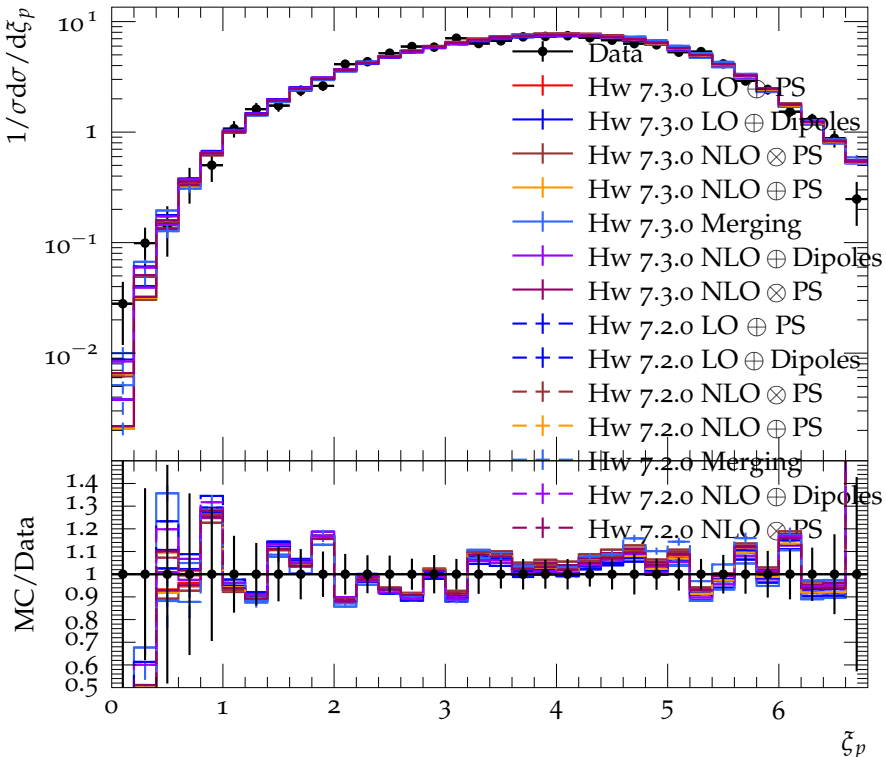
Log of scaled momentum distribution at E_{\text{CMS}} = 161.3 \text{ GeV}
