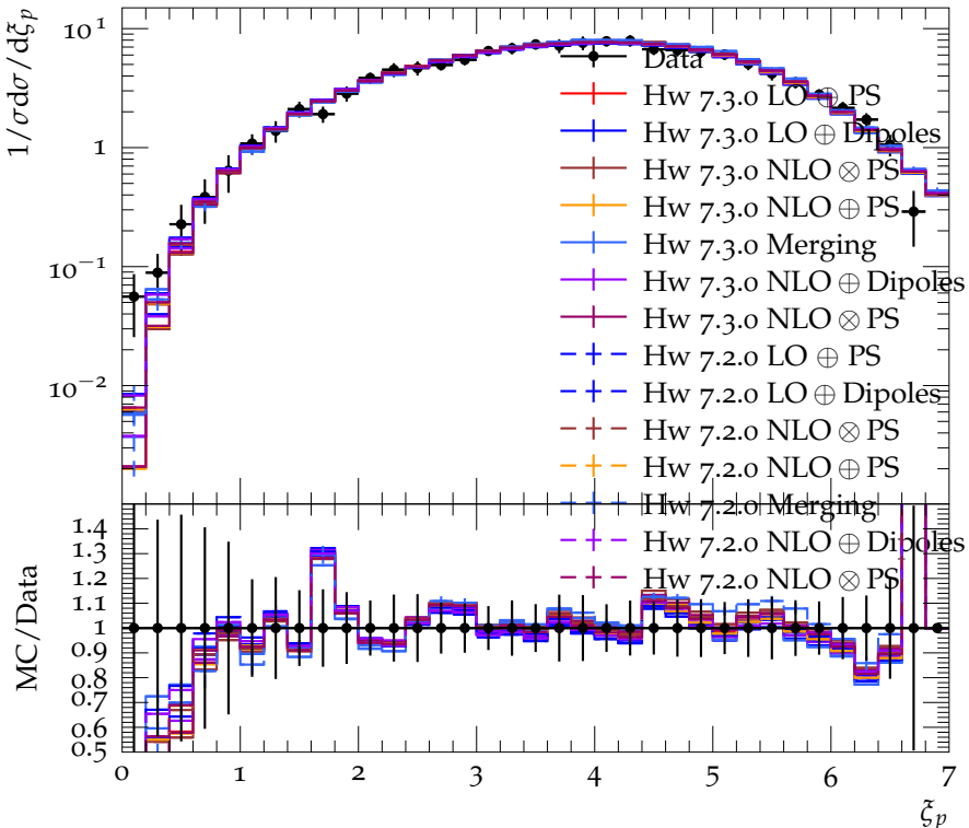
Log of scaled momentum distribution at E_{\text{CMS}} = 172.3 \text{ GeV}
