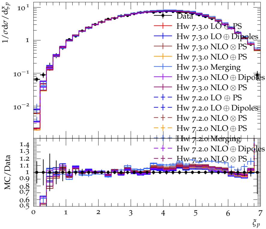
Log of scaled momentum distribution at E_{\text{CMS}} = 188.6 GeV
