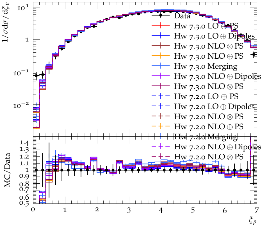
Log of scaled momentum distribution at E_{\text{CMS}} = 200.2 \text{ GeV}
