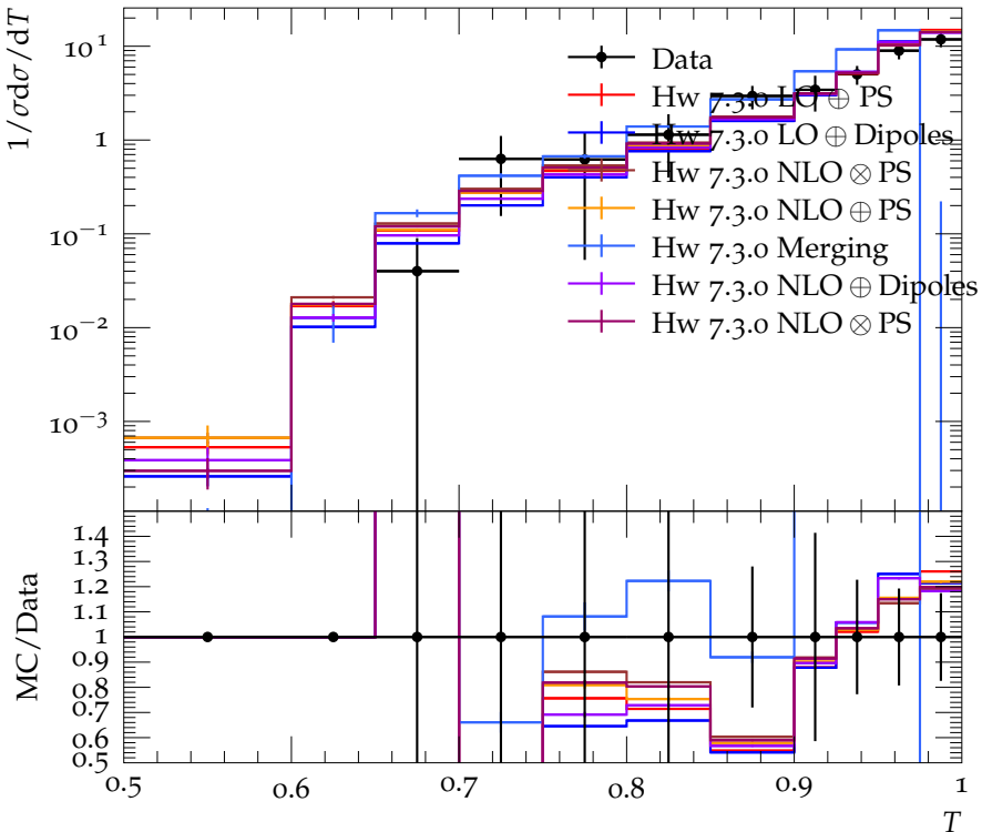
Thrust, bottom events, at E_{\text{CMS}} = 197 \text{ GeV}
